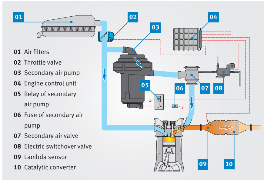
Block diagram of secondary air system (pneumatically actuated)
