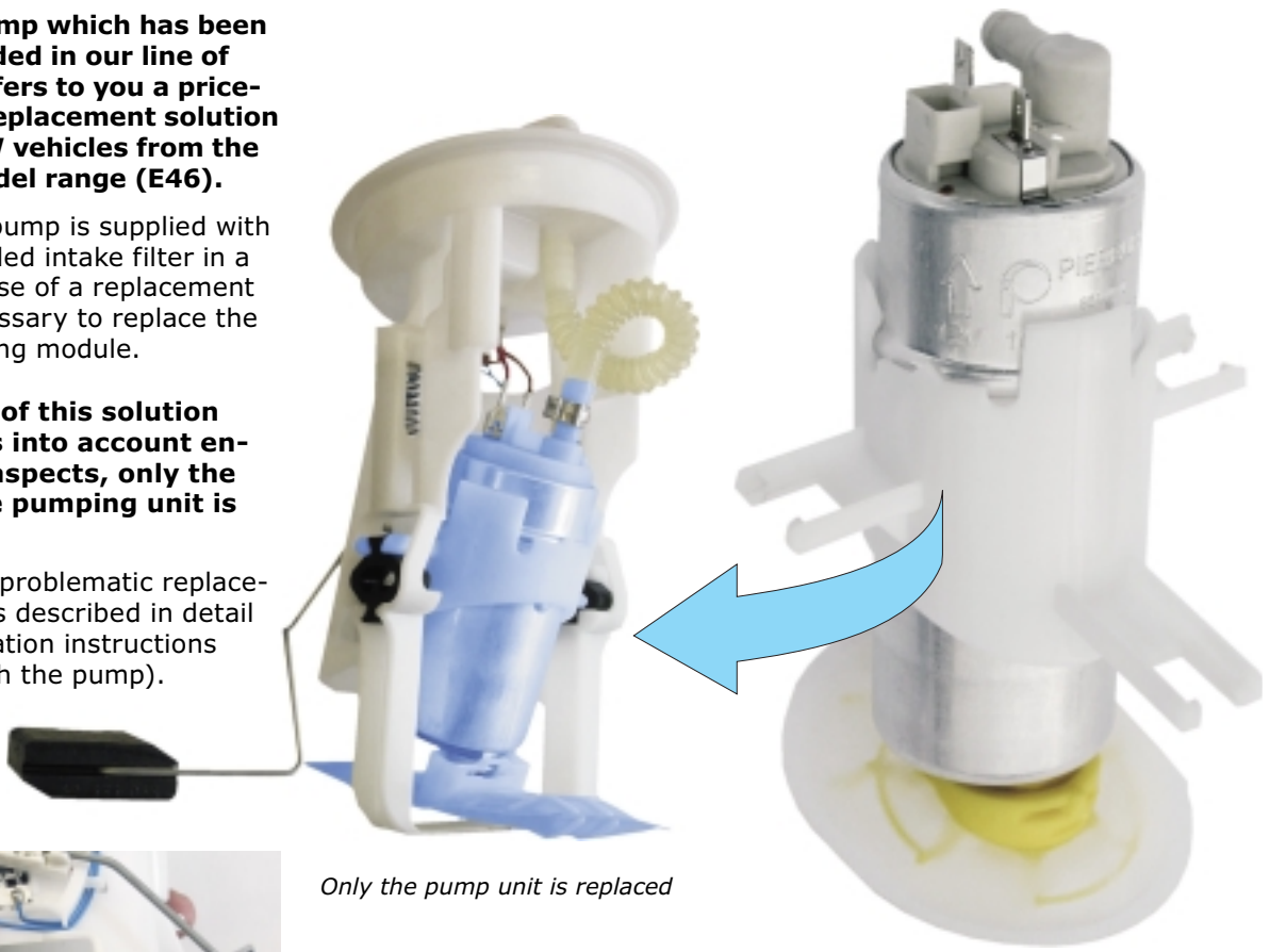
Pierburg replacement pump
