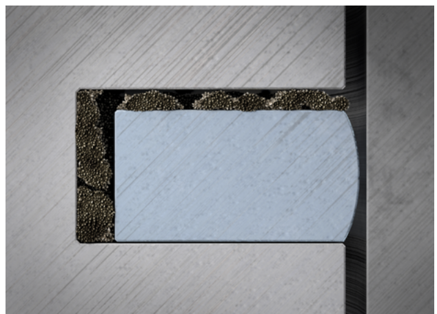
Fig. 3: Blocked piston rings
