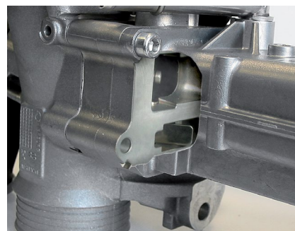
Bypass flap in the EGR cooler (cut away view)
